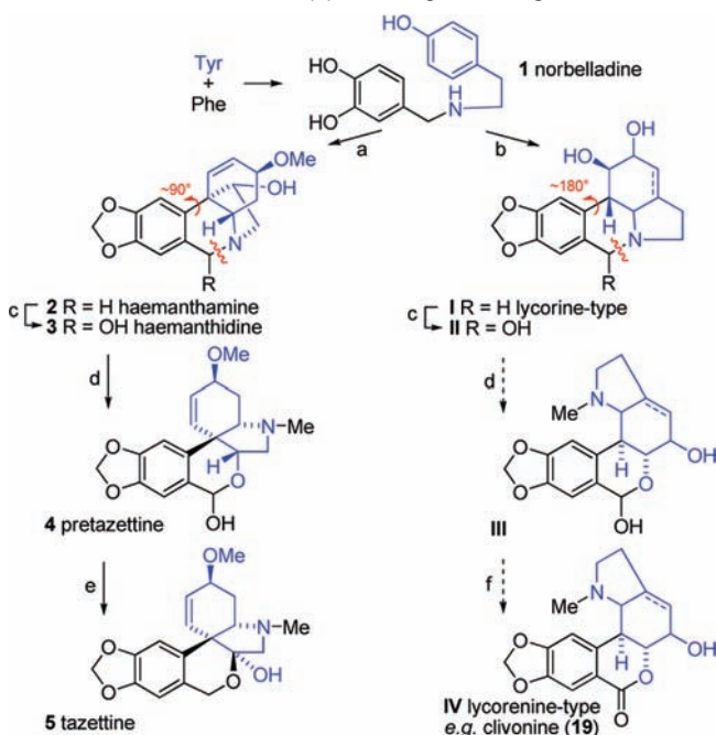
Scheme 1. Outline Biosynthesis of Tazettine and Lycorenine-Type Alkaloids from Norbelladine ( 1 ) via “Ring-Switching” a
